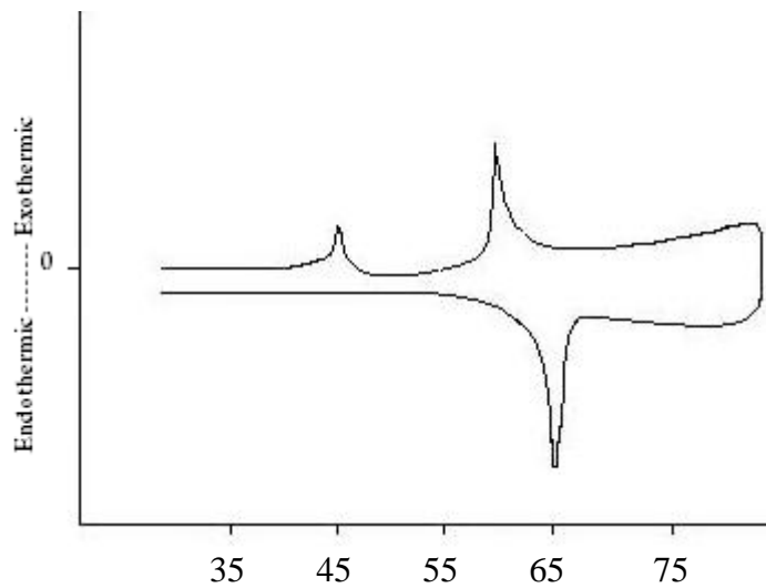
Figure 1 DSC graph transition points of 4- n – octyloxy – 2,3,5,6, tetra methyl -4 – octyloxy azo benzene
